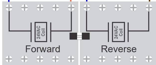
Motor 1 Contactor
