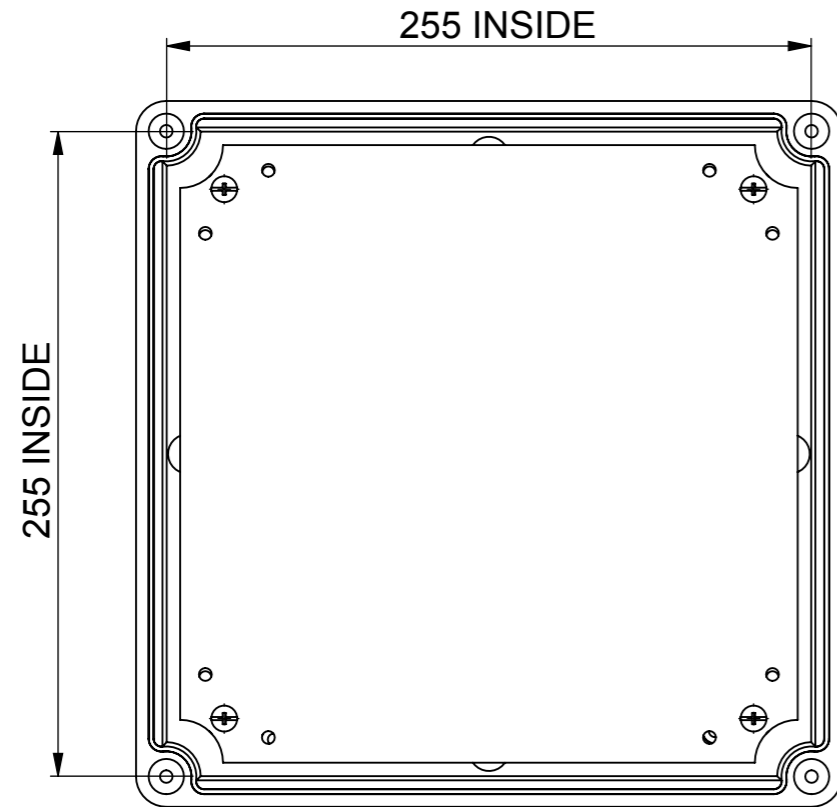
TOP VIEW (LID WAS HIDDEN TO SHOW INSIDE)
