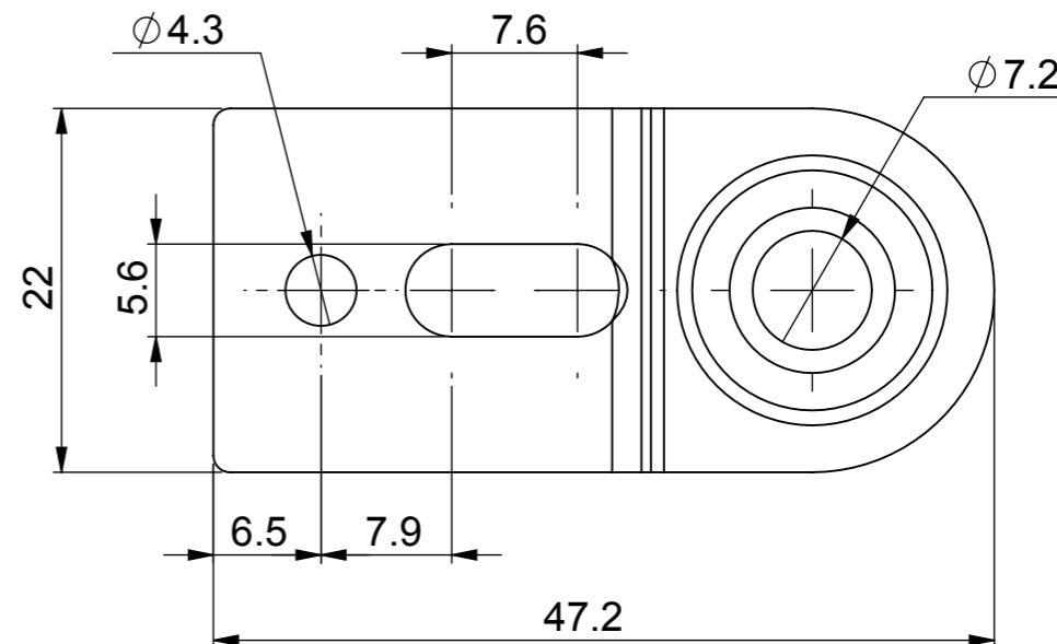
ITEM NO.6: MOUNTING BRACKET
