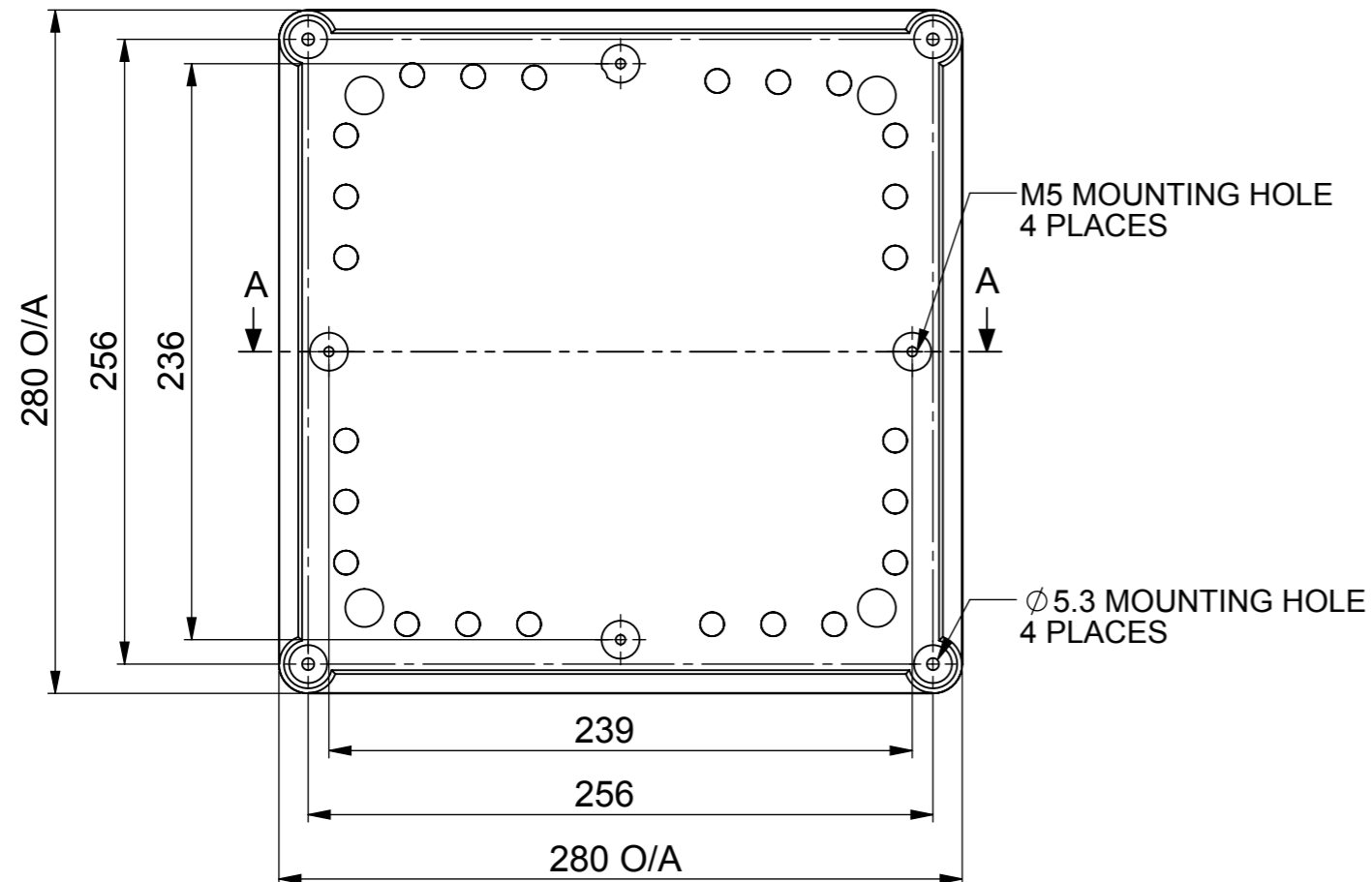
BACK VIEW
