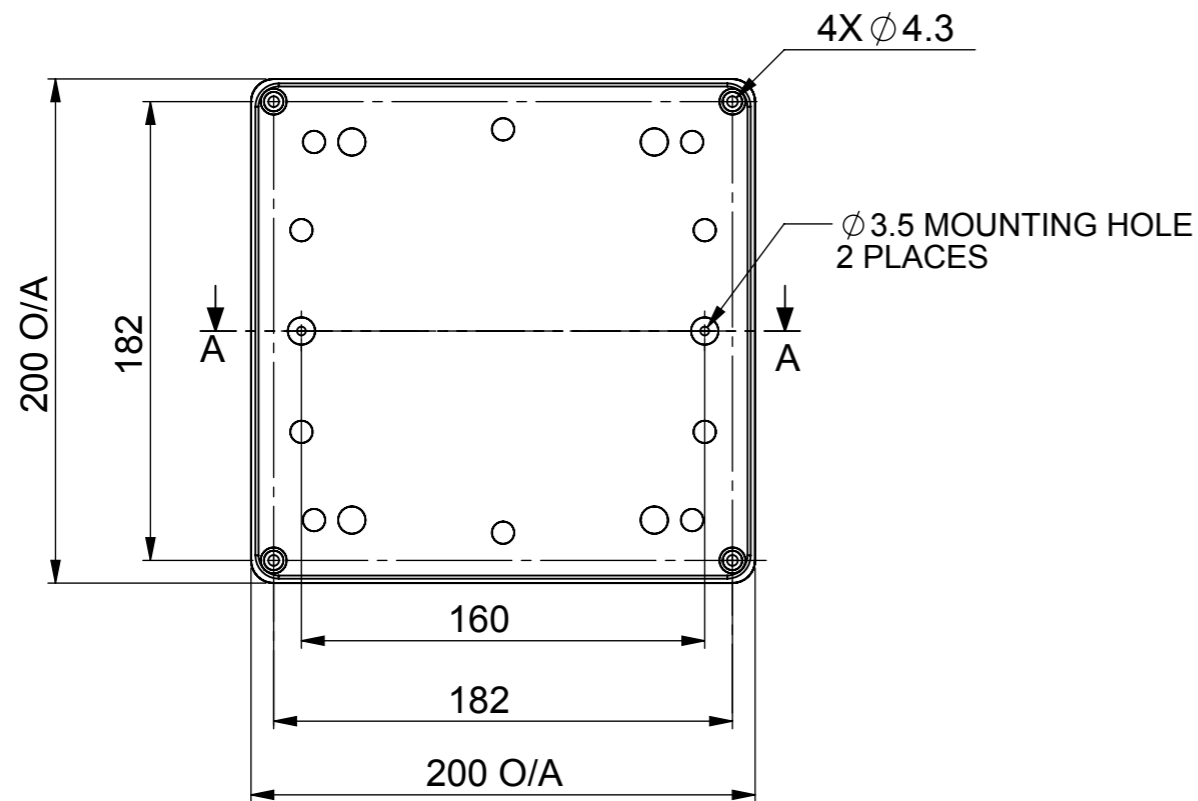
BACK VIEW
