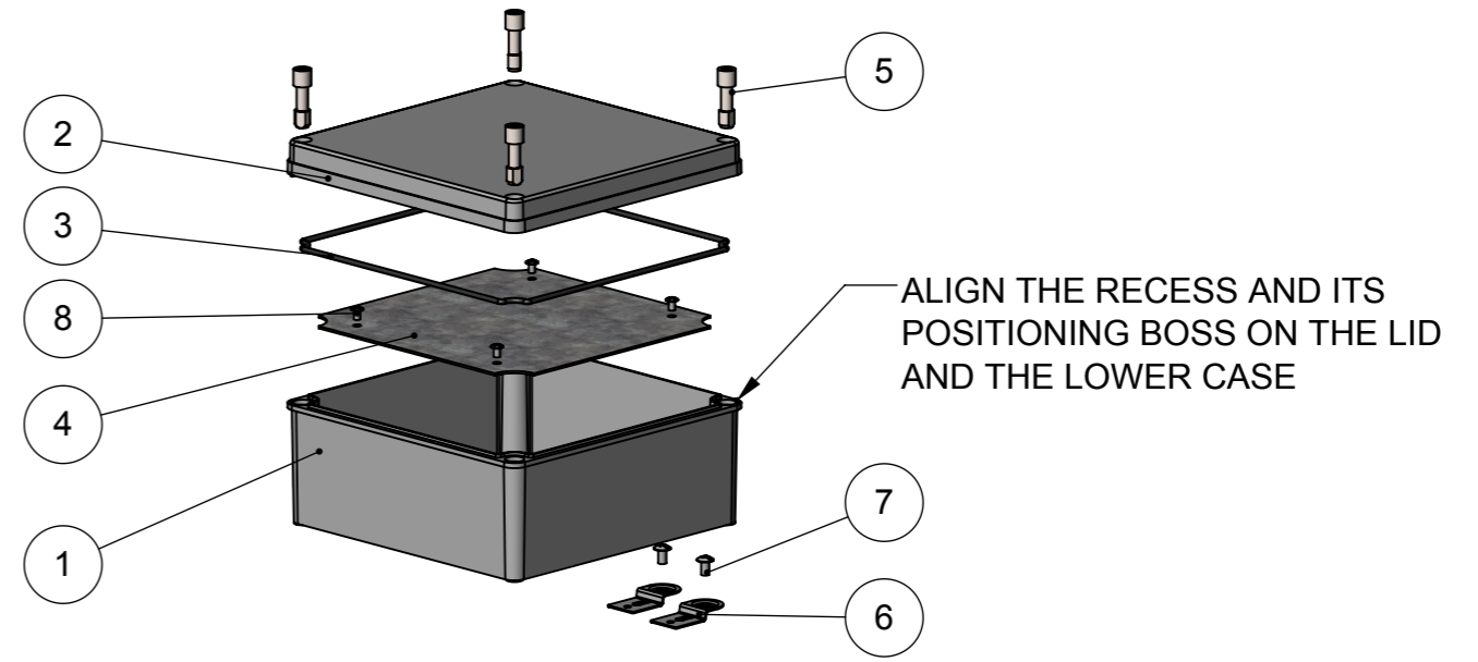
SCALE 1:5
