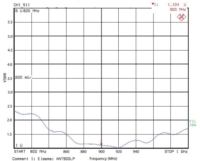
Typical VSWR Response
